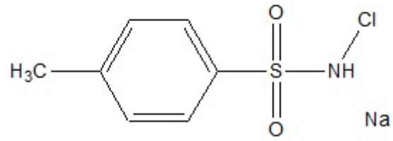
Chloramine-T
